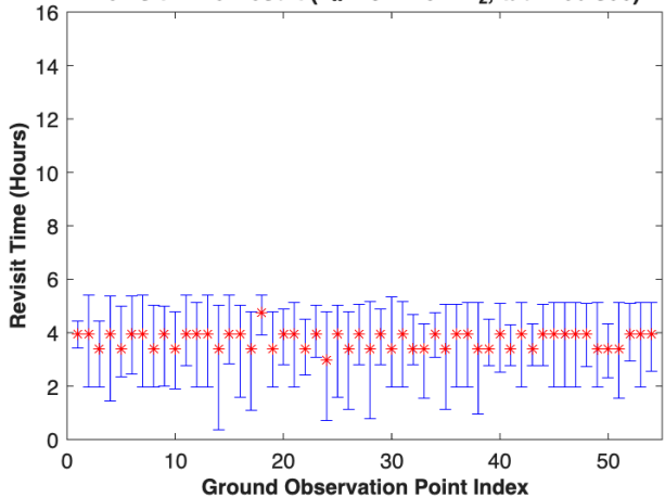
Revisit Time Result ( L_\infty BCD from L_2 , \tau = 30 sec)
