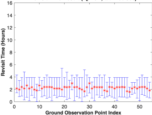
Revisit Time Result ( L_2 BCD, \tau = 30 sec)
